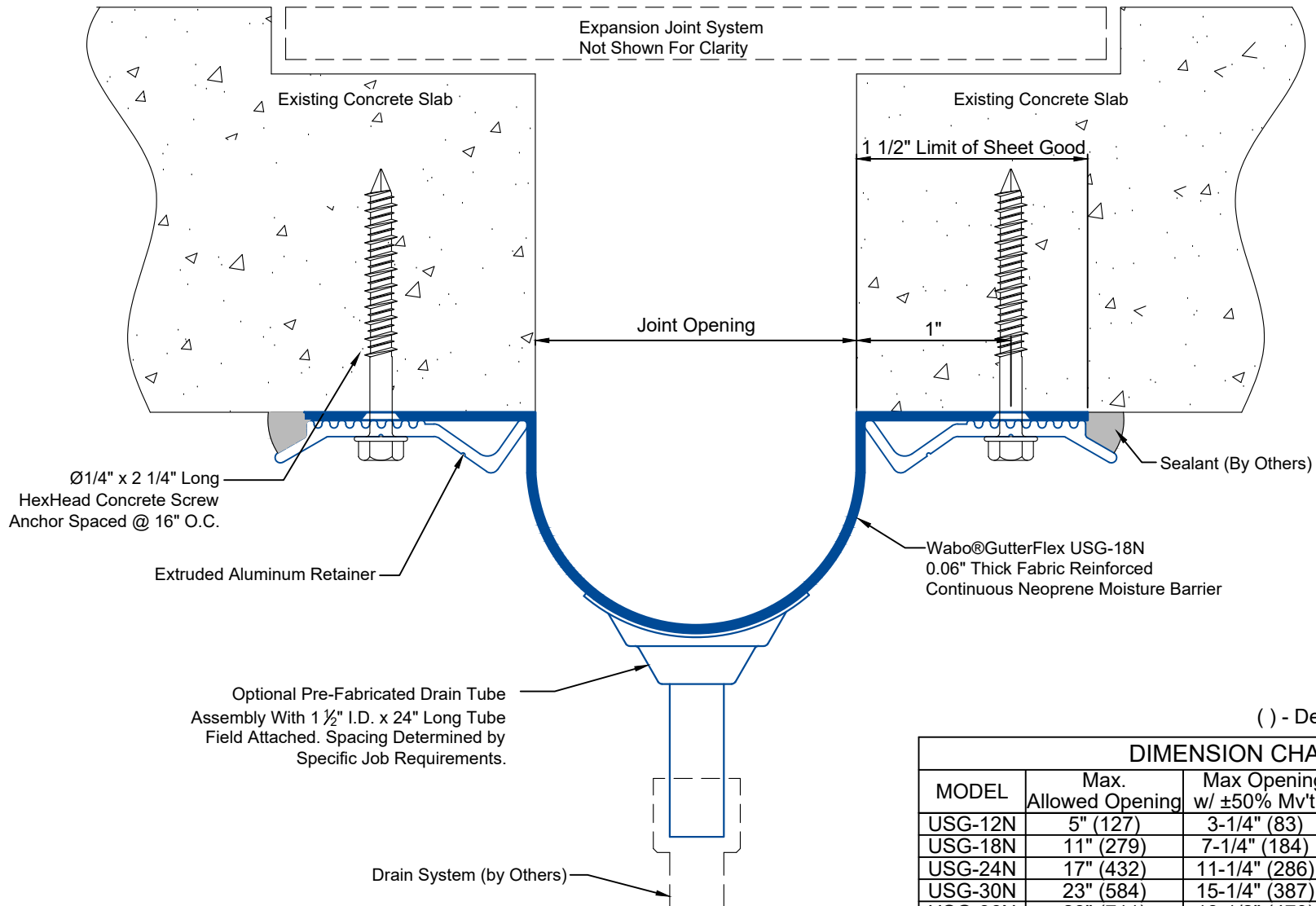
TYPICAL GUTTER SECTION UNDER SLAB APPLICATION
