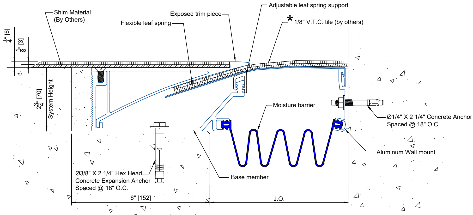
Typical Detail Floor to Wall - Tile Condition
