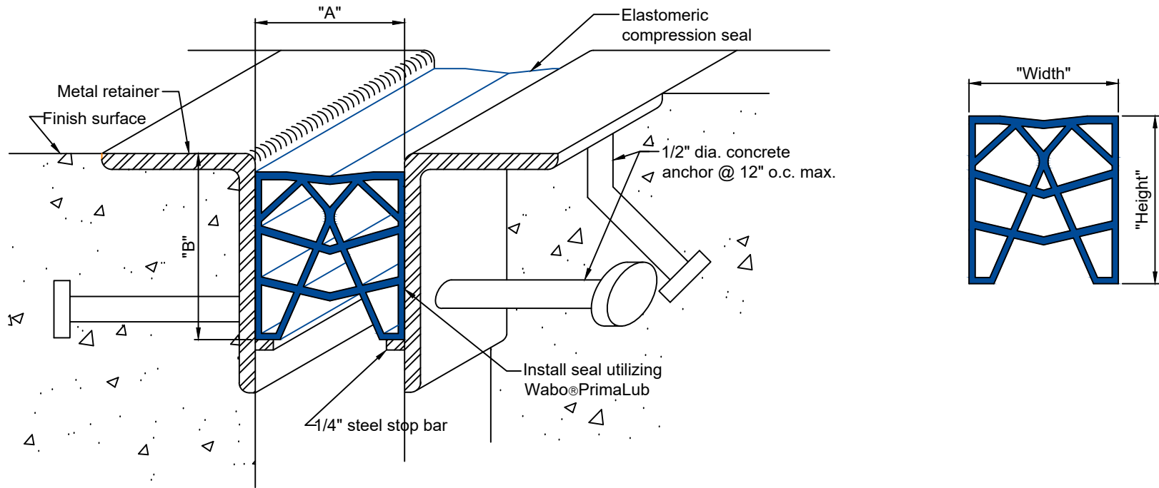
"WA" Profile Armored Blockout Condition
