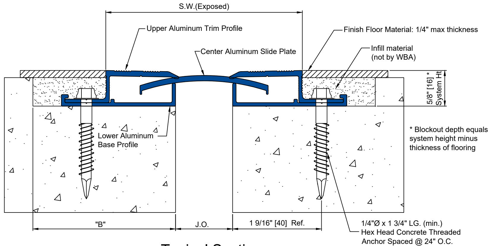
Typical Section Floor To Floor
