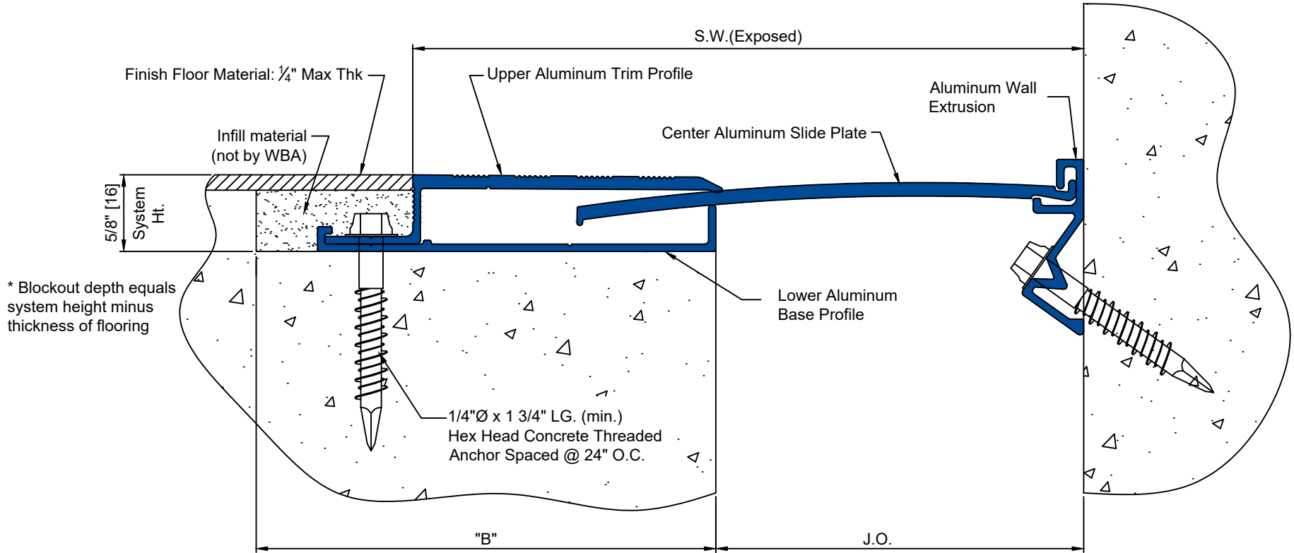
Typical Section Floor To Wall
