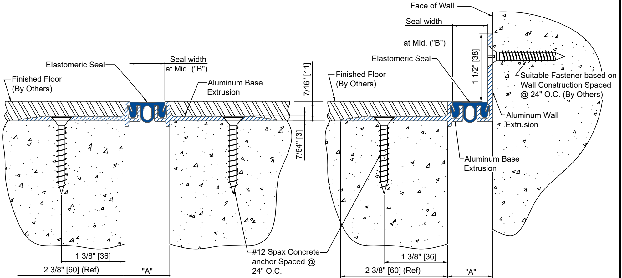
CWFC-100C DETAIL FLOOR TO WALL CONDITION
