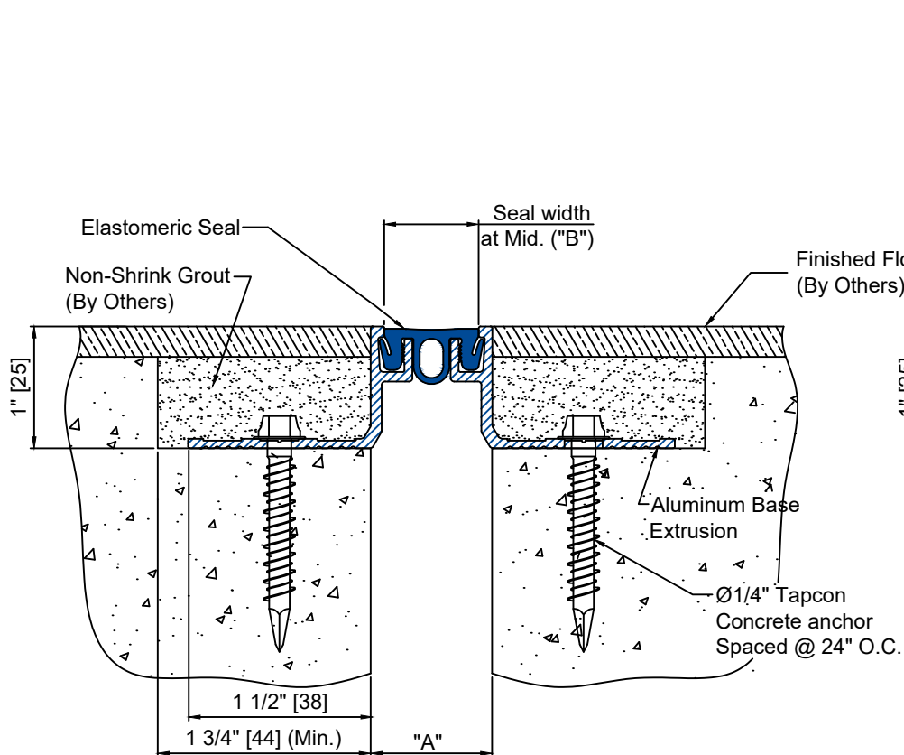
CWFF-100 DETAIL FLOOR TO FLOOR CONDITION
