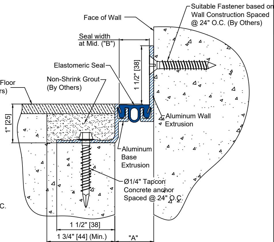
CWFF-100C DETAIL FLOOR TO WALL CONDITION
