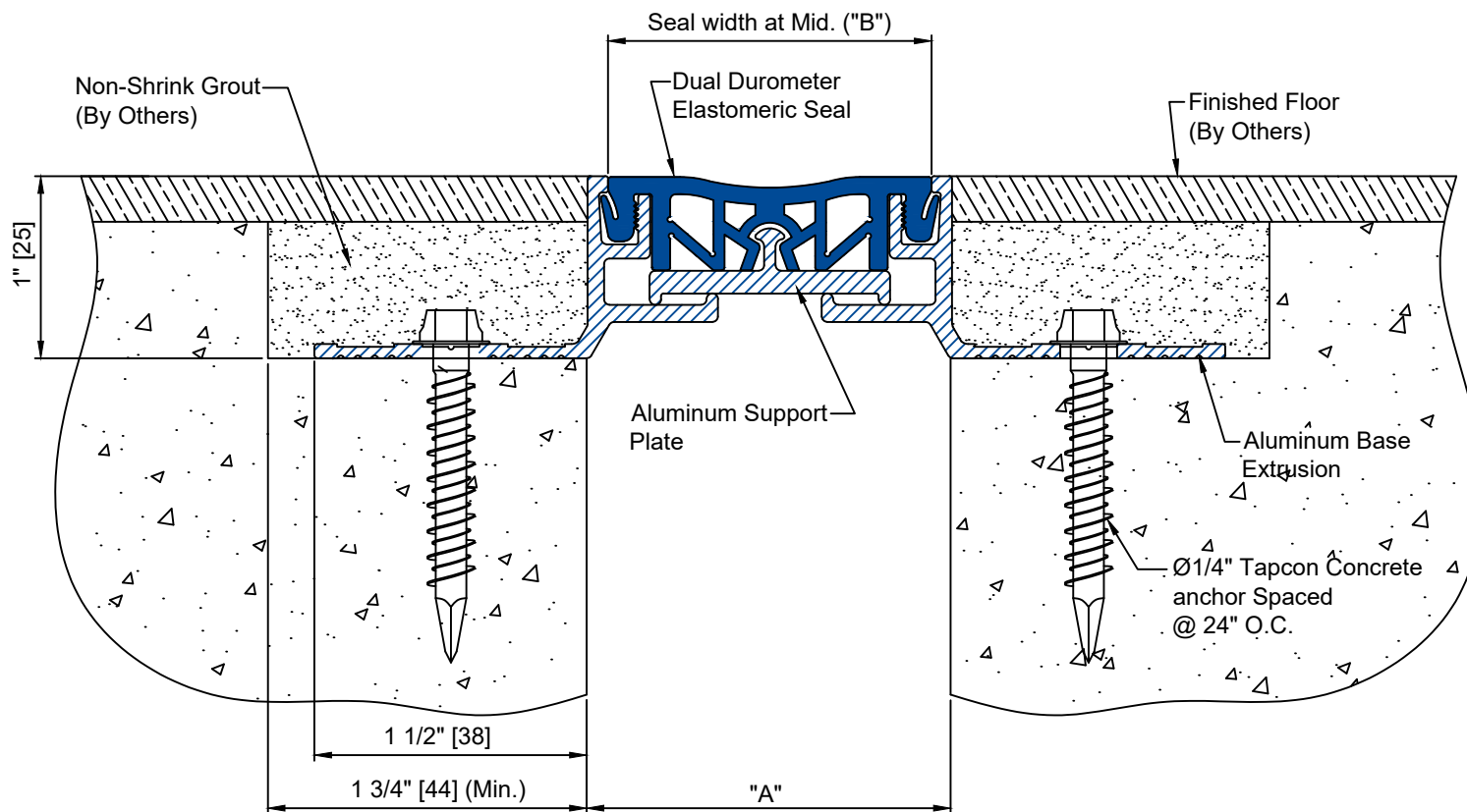
CWFF-200 thru 300 DETAIL FLOOR TO FLOOR CONDITION
