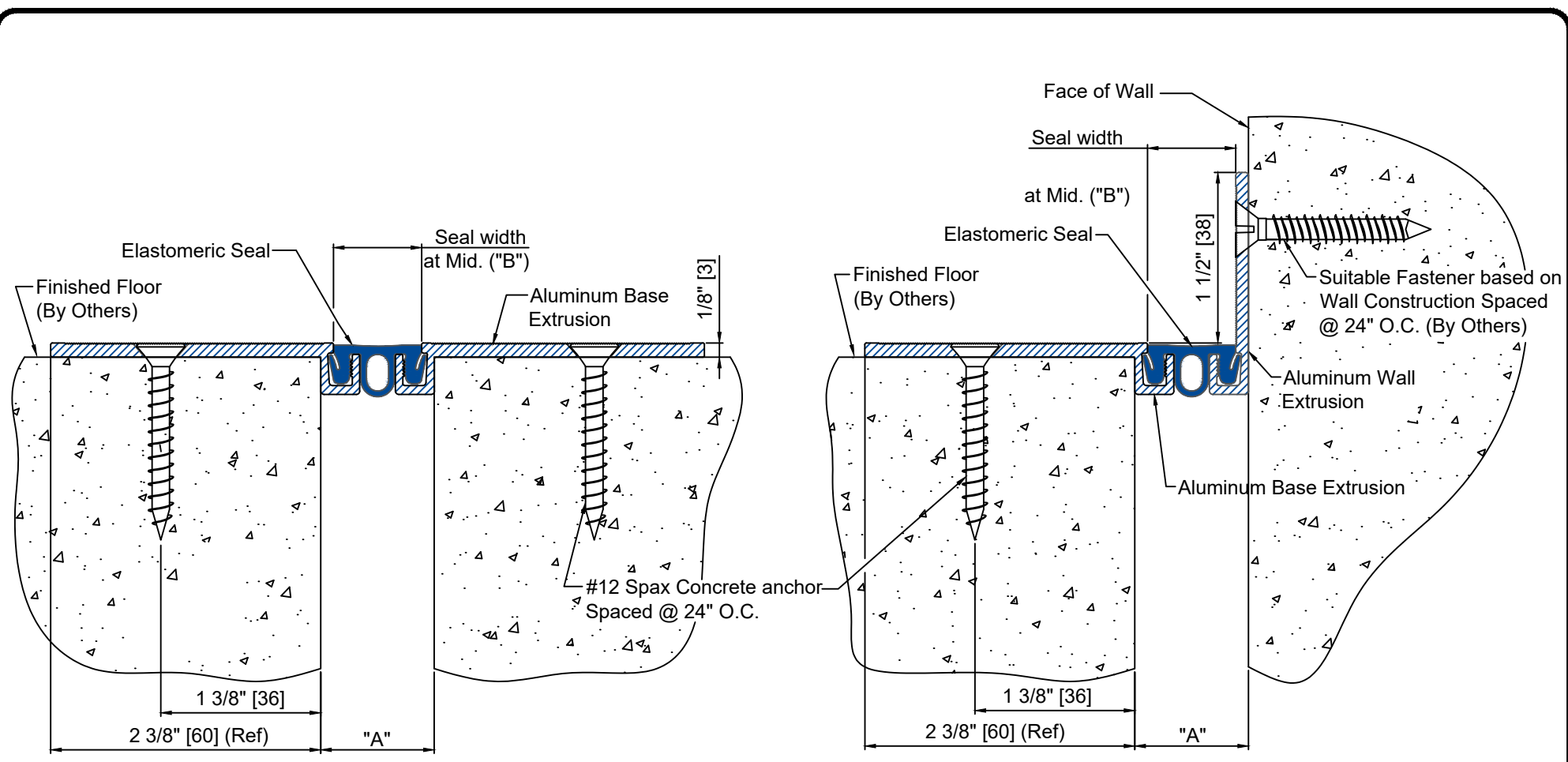
CWFT-100 DETAIL FLOOR TO FLOOR CONDITION
