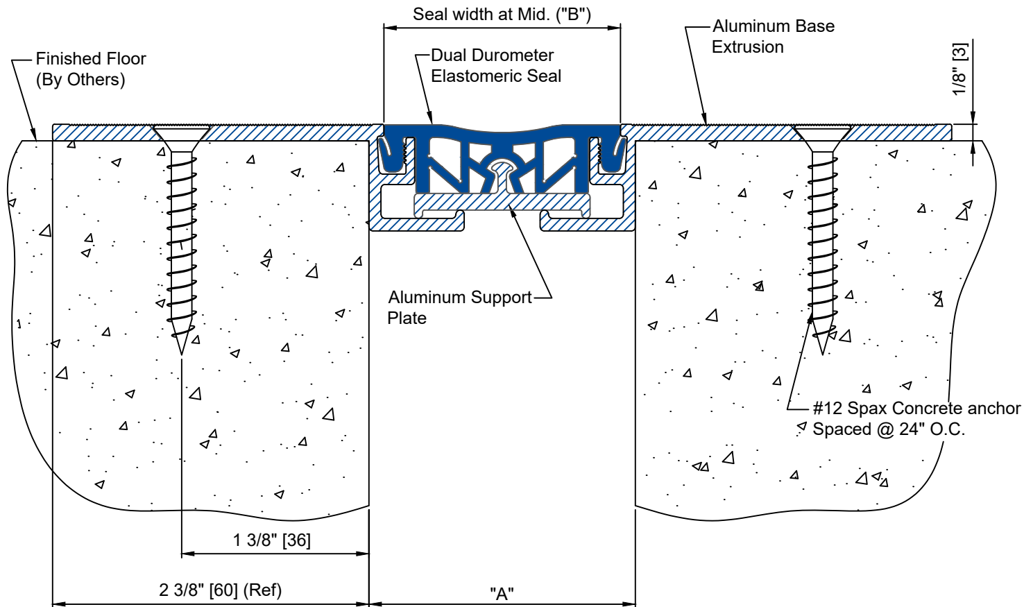
CWFT-200 thru 300 DETAIL FLOOR TO FLOOR CONDITION
