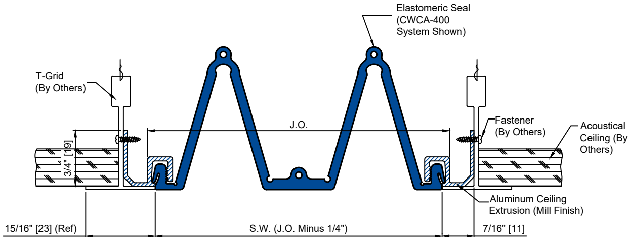
Standard Detail
