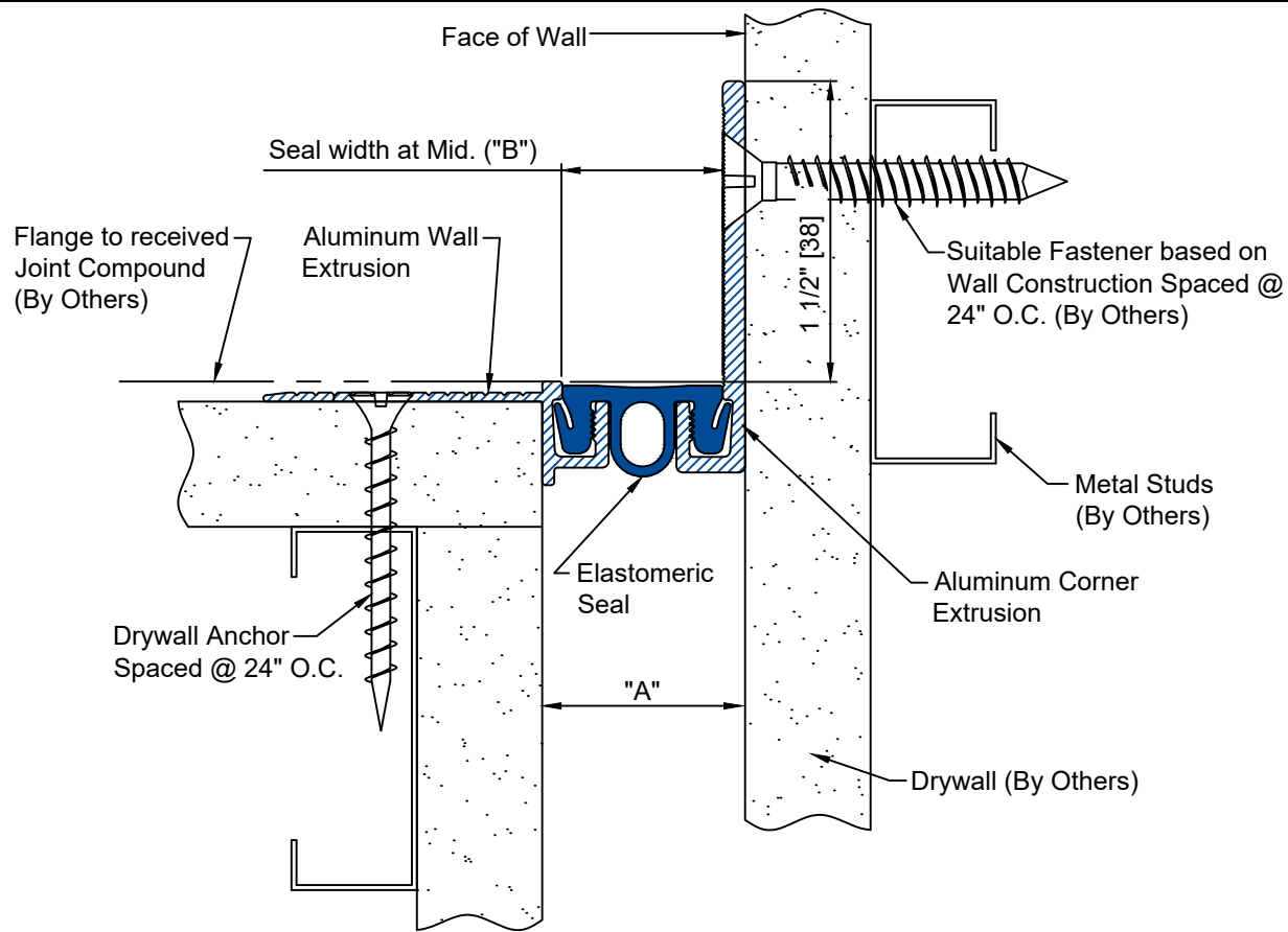
CWWE-100 DETAIL WALL TO WALL CONDITION
