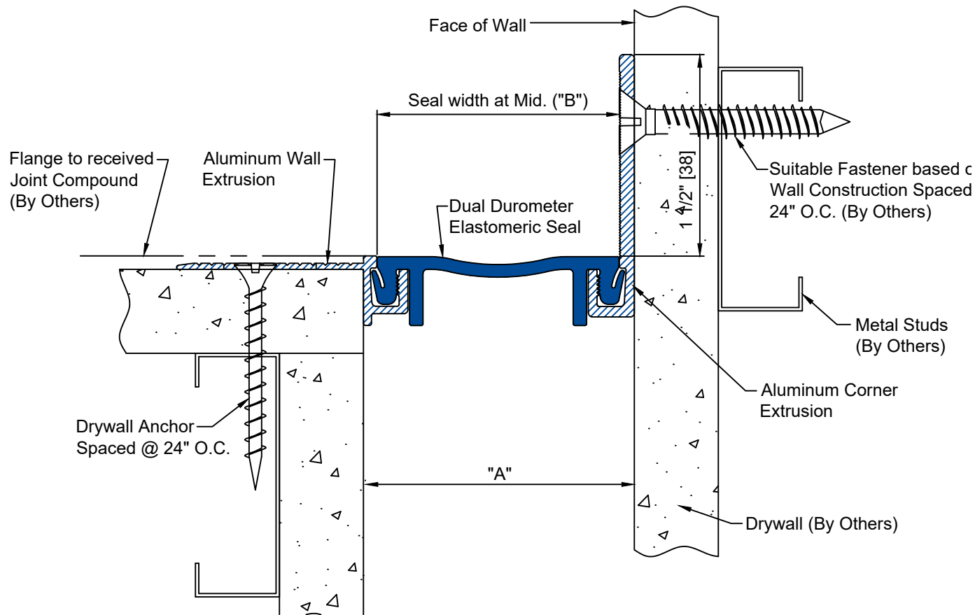
CWWE-200 thru 300 DETAIL WALL TO WALL CONDITION
