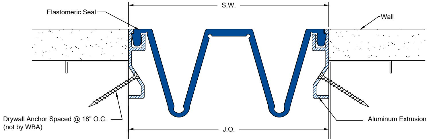
CWWF-400/500/600 typical section wall to wall application gypsum shown - others similar
