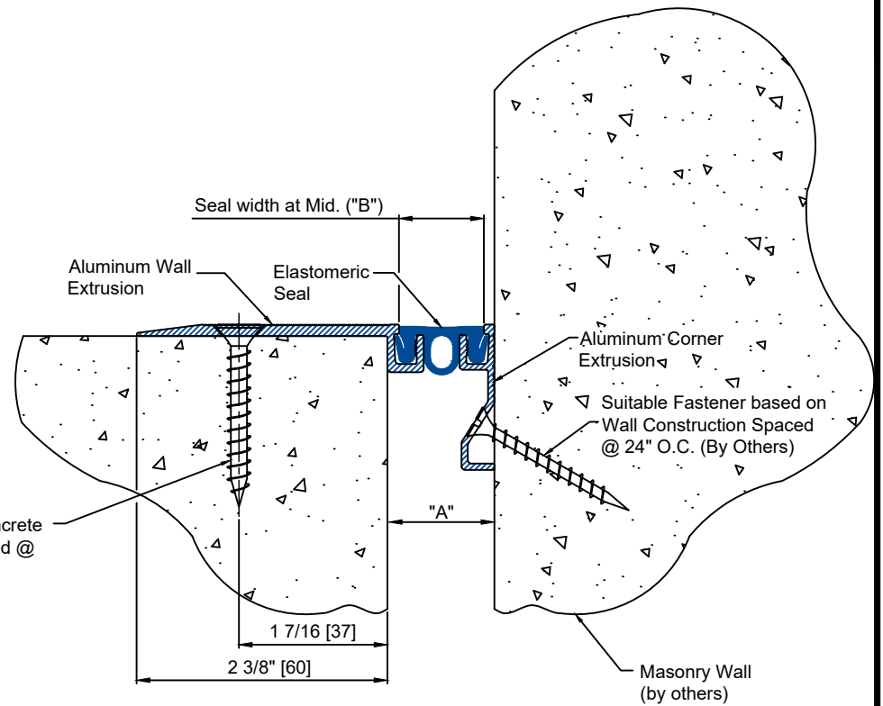
CWWM-100C DETAIL WALL TO WALL CORNER CONDITION
