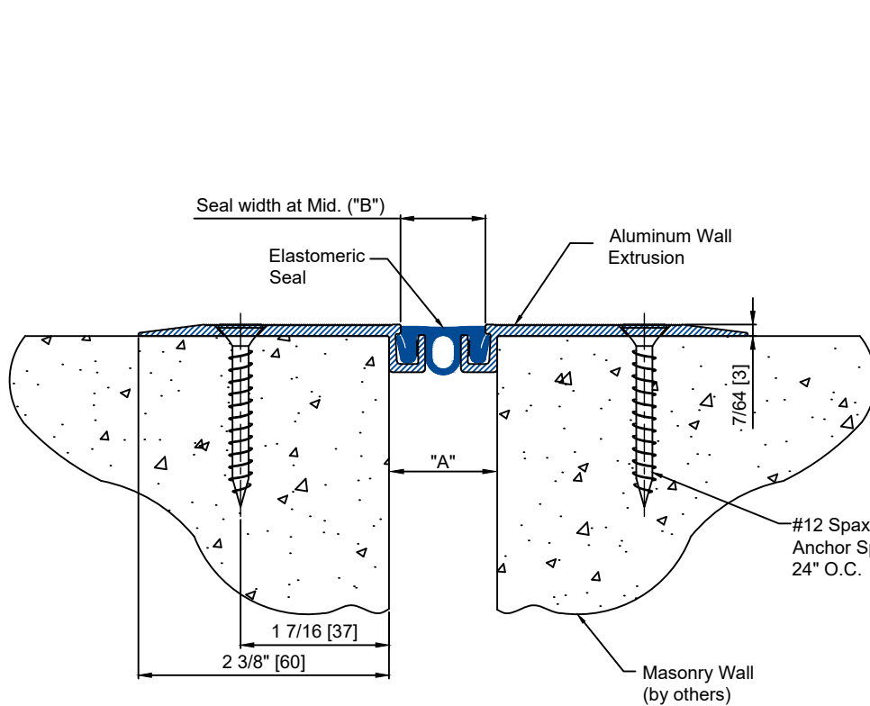
CWWM-100 DETAIL WALL TO WALL CONDITION
