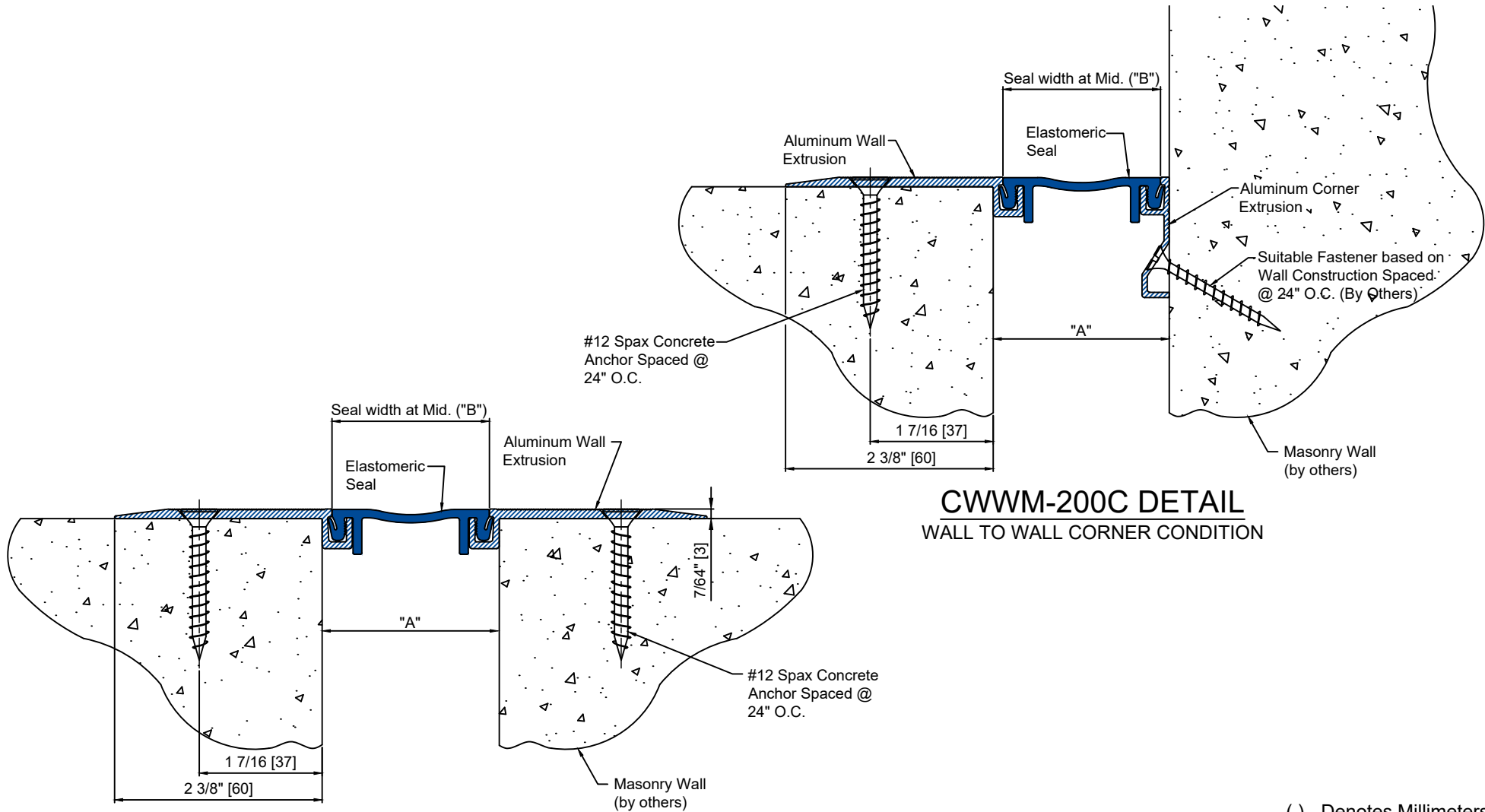
CWWM-200 DETAIL WALL TO WALL CONDITION
