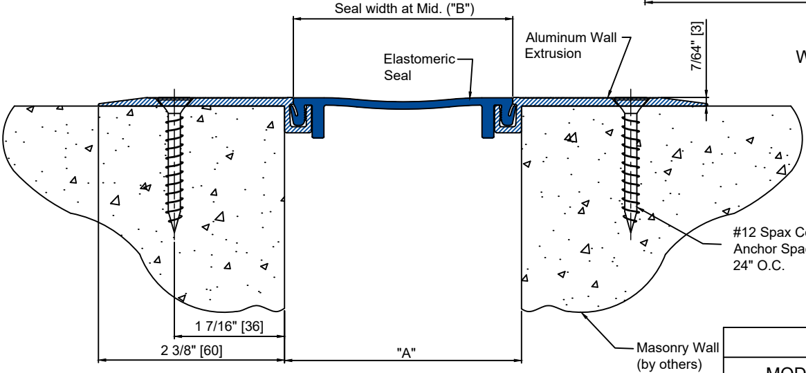
CWWM-300 DETAIL WALL TO WALL CONDITION
