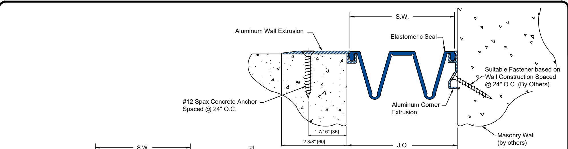
CWWM-400C DETAIL Wall to Wall Condition
