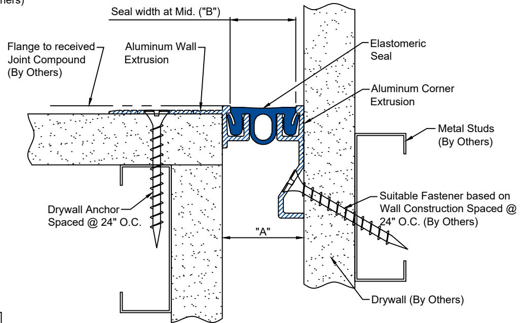
CWWS-100C DETAIL WALL TO WALL CORNER CONDITION
