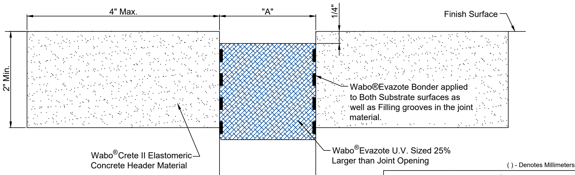
TYPICAL SECTION
