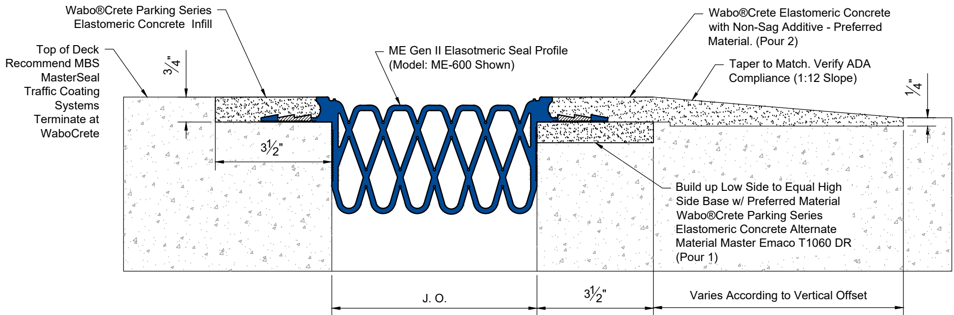
STANDARD VERTICAL OFFSET DETAIL TYP. SECTION
