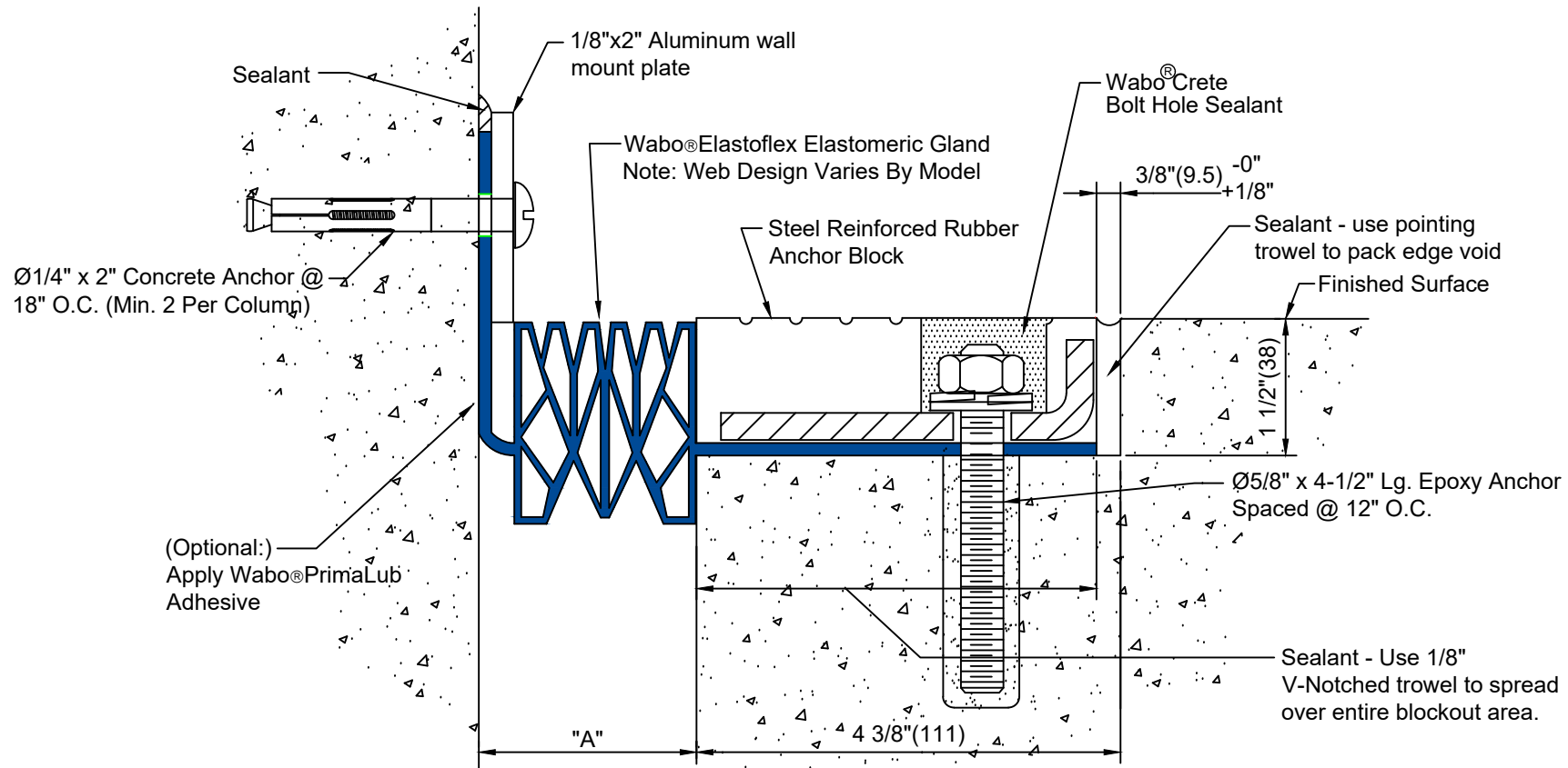
MODEL EFJ-C SLAB-TO-WALL CONDITION
