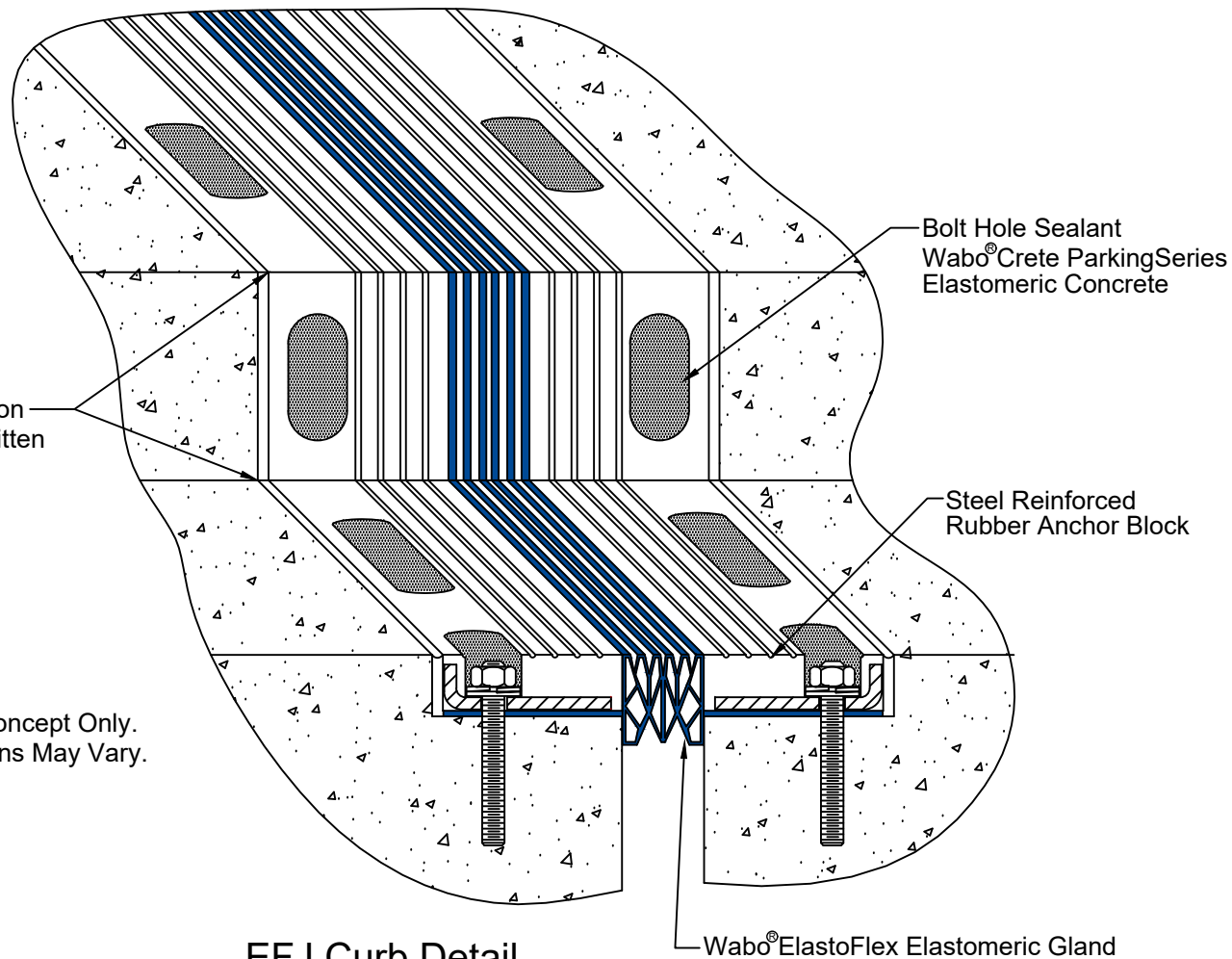
EFJ Curb Detail
