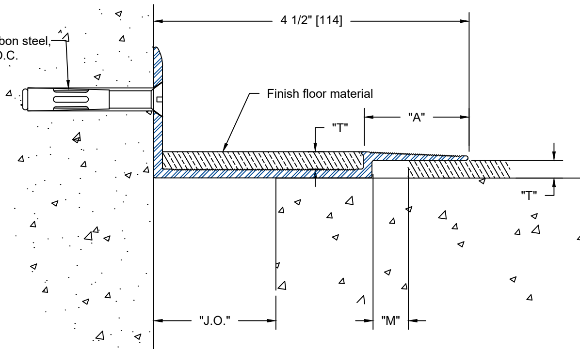
Typical Section Floor to Floor Condition
