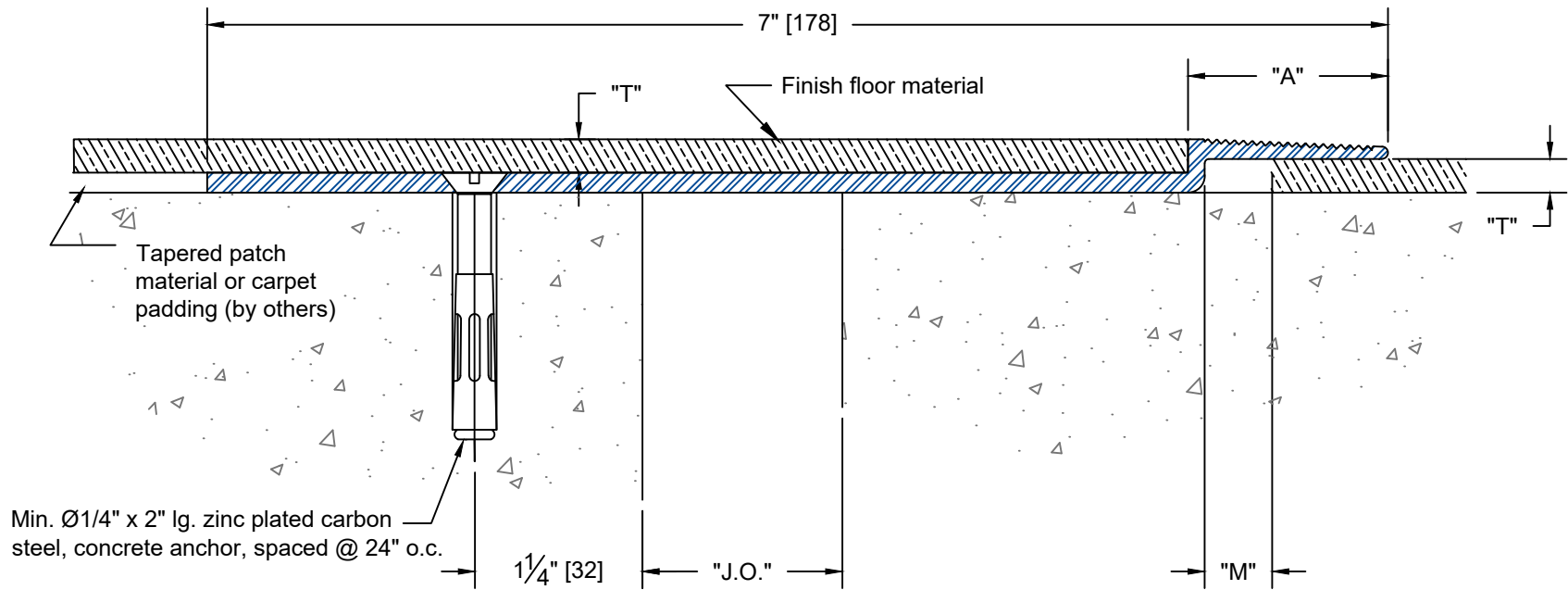
Typical Section Floor to Floor Condition
