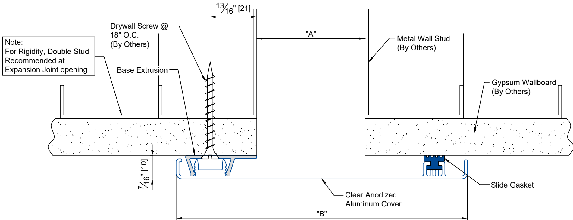
TYPICAL SECTION WALL TO WALL CONDITION NOT TO SCALE
