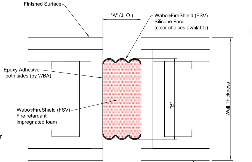
WaboFireShield FSV Detail Gypsum to Gypsum Condition NOT TO SCALE
