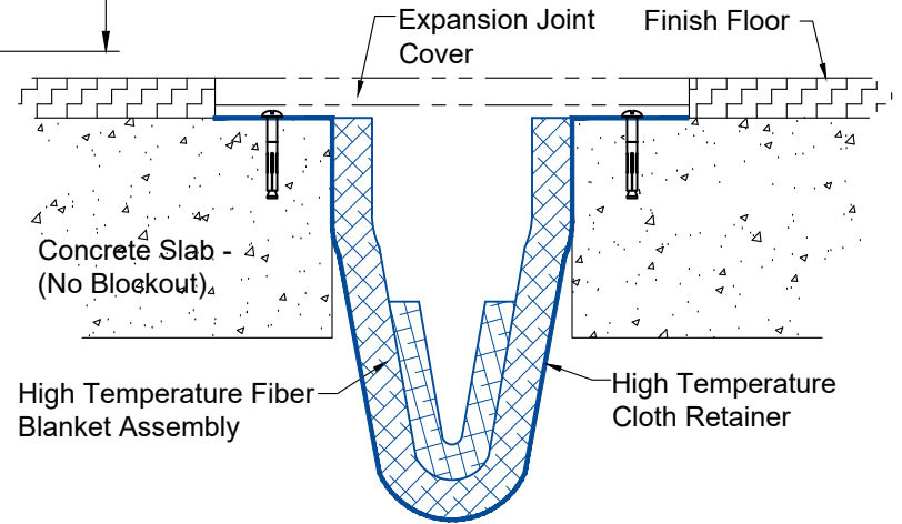
Detail A Surface Mounted Condition
