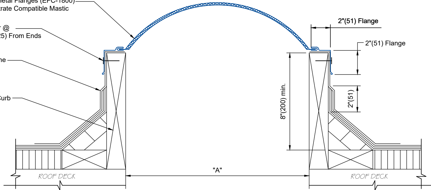
ECF-1800 DETAIL
