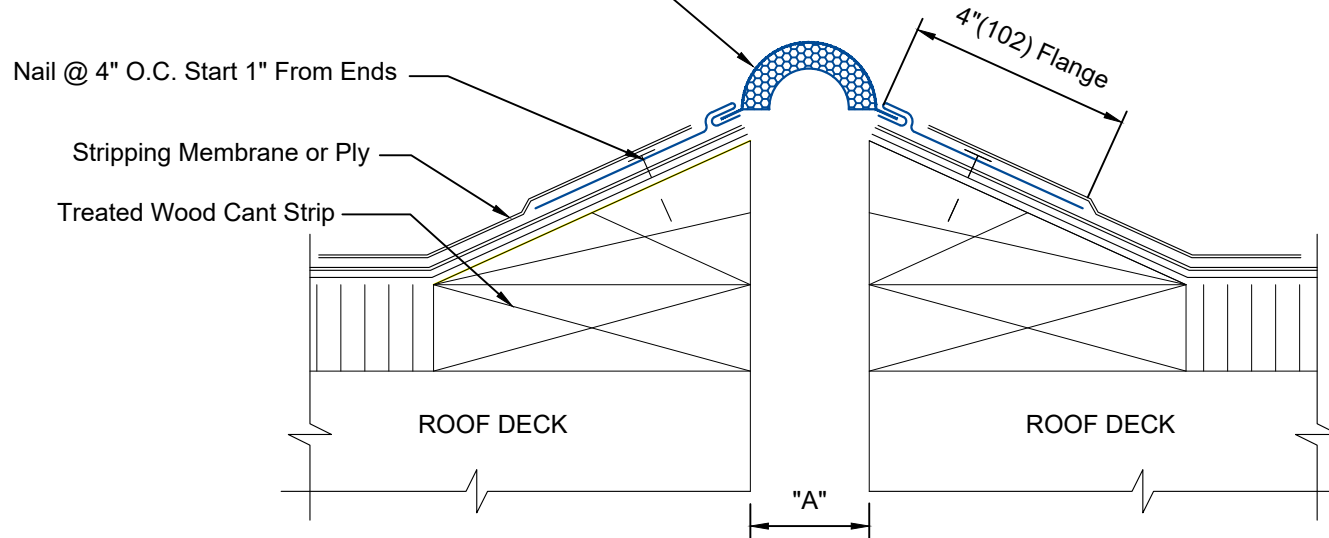
EEJ-100 DETAIL
