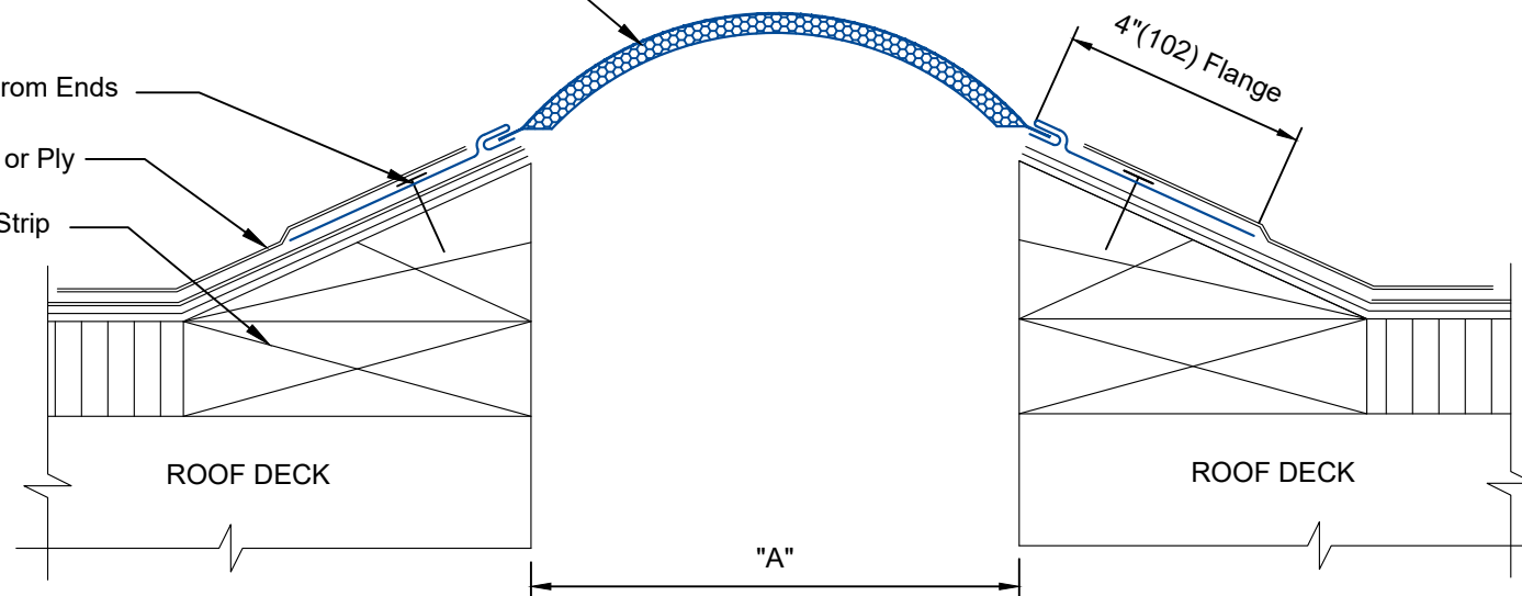
EEJ-1200 DETAIL
