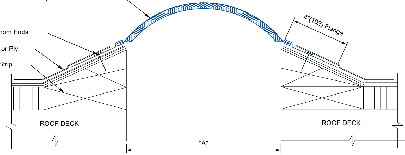
EEJ-1600 DETAIL
