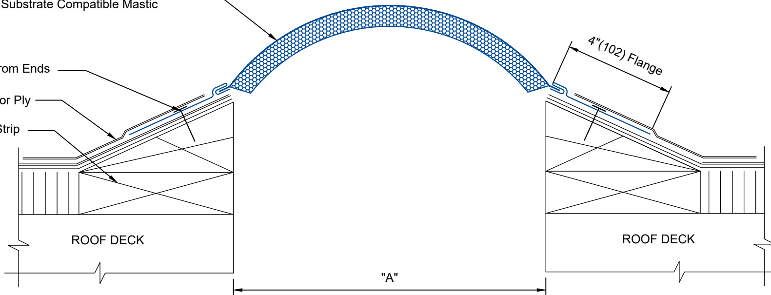
EEJ-2000 DETAIL
