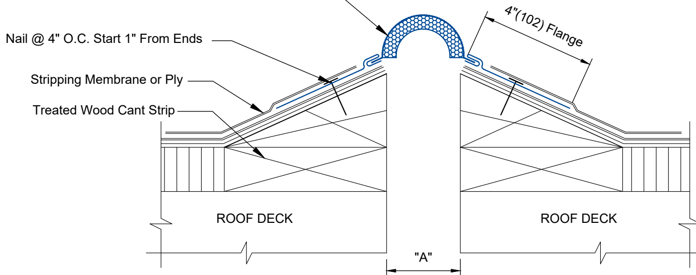
EEJ-200 DETAIL
