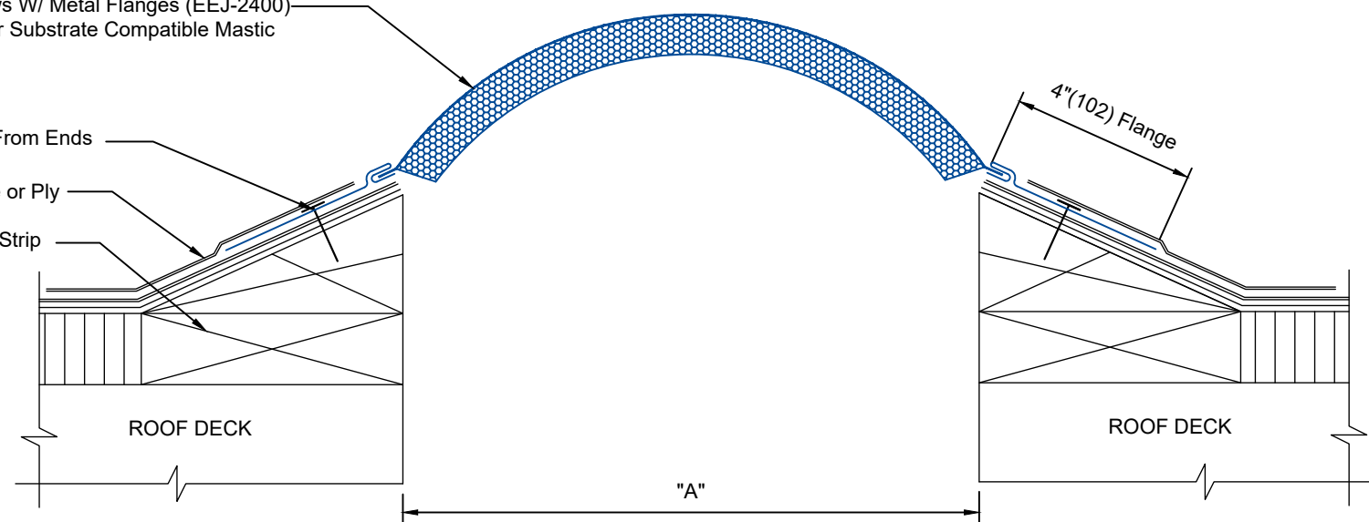
EEJ-2400 DETAIL
