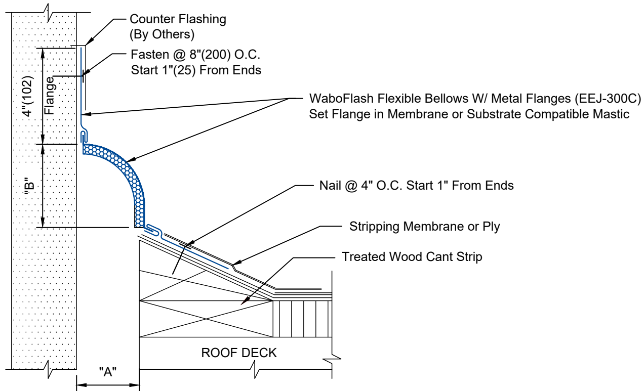
EEJ-300C DETAIL
