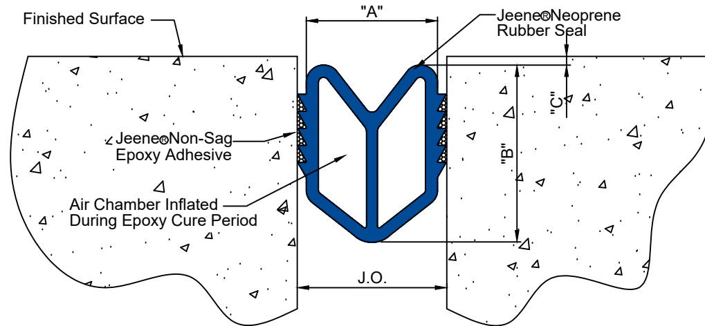
"W" PROFILE SLAB-TO-SLAB CONDITION
