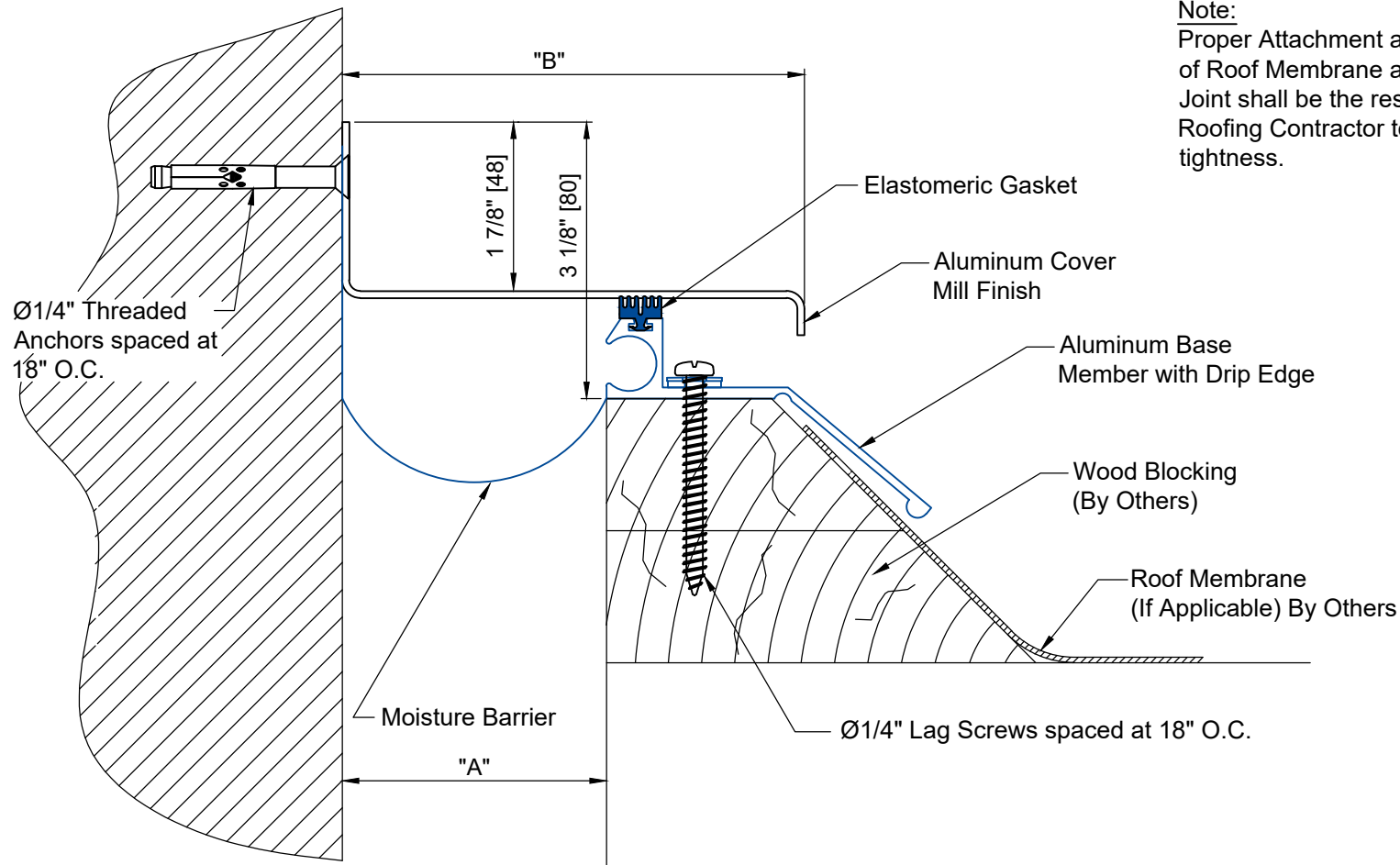
RFC-200C THRU RFC-800C WALL-TO-ROOF CONDITION
