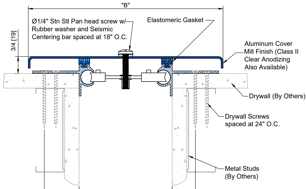
WFI-200 Thru WFI-2400 DETAIL WALL-TO-WALL INTERIOR CONDITION
