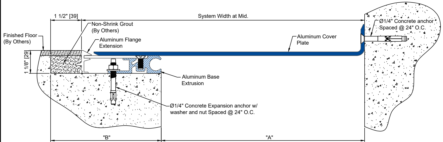
FNB-1000C DETAIL Floor to Wall Condition
