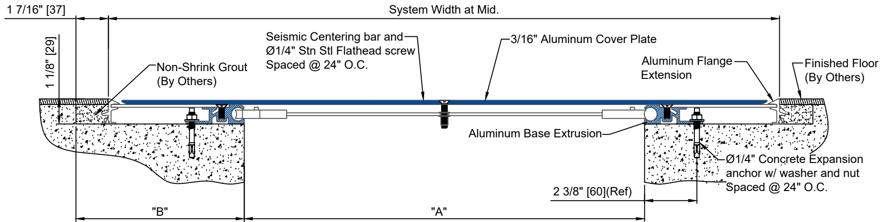
FNB-1800 DETAIL Floor to Floor Condition
