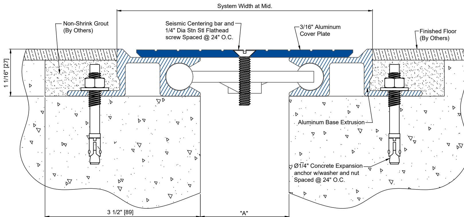
FNB-200 DETAIL FLOOR TO FLOOR CONDITION
