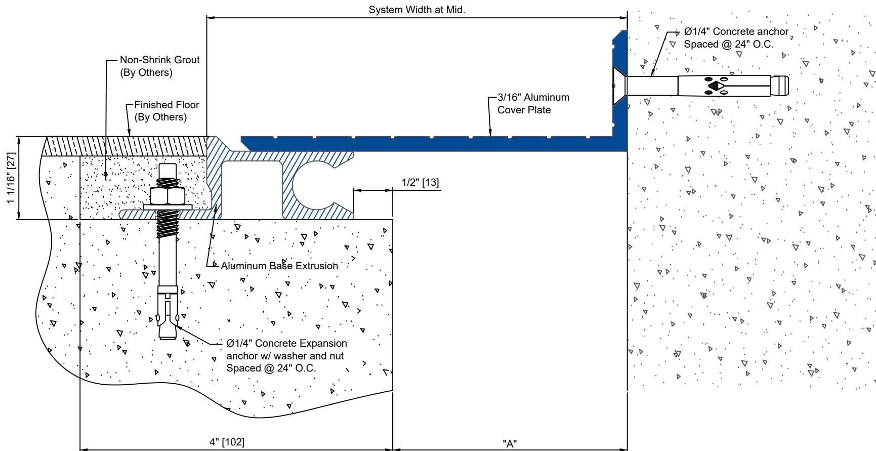
FNB-300C DETAIL FLOOR TO WALL CONDITION
