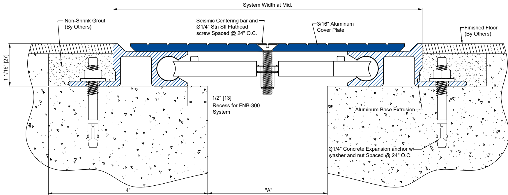
FNB-300 DETAIL FLOOR TO FLOOR CONDITION
