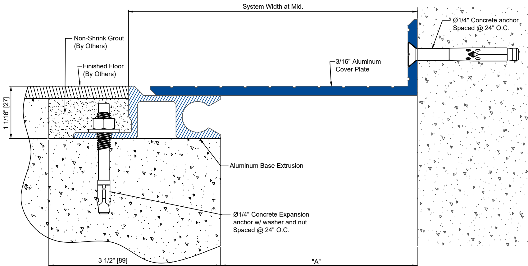
FNB-400C DETAIL FLOOR TO WALL CONDITION
