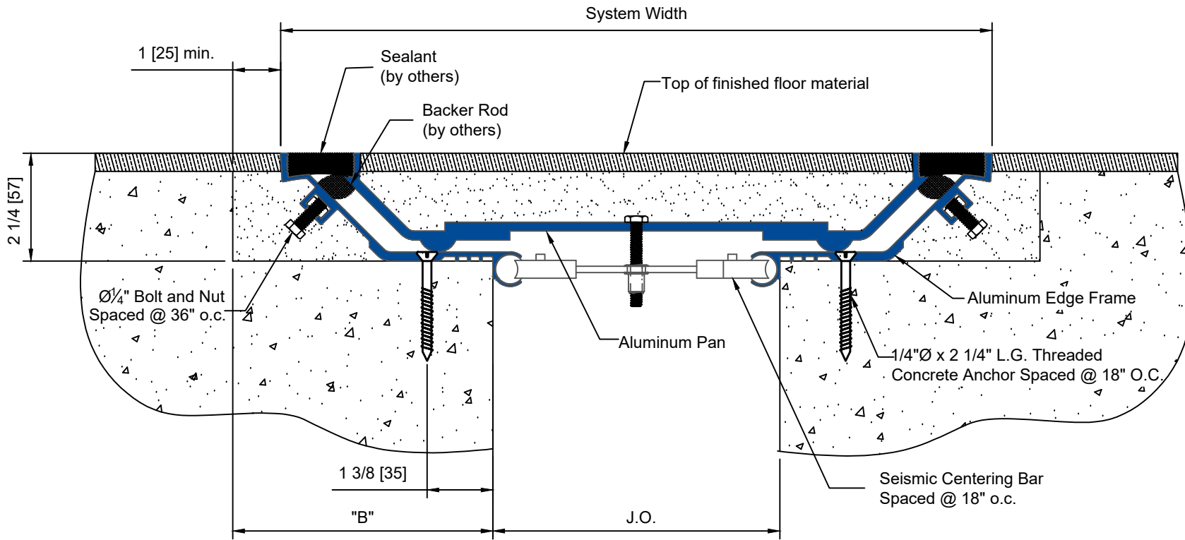
Typical Section Floor To Floor
