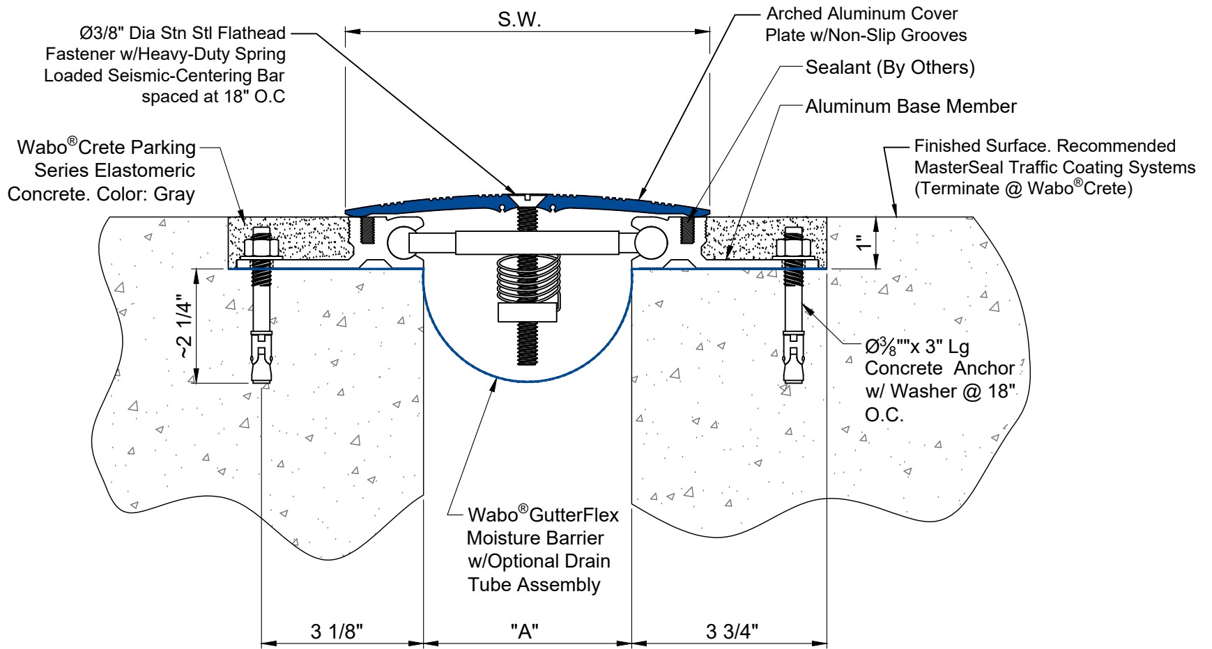
APS-II 200/400 Floor to Floor Condition
