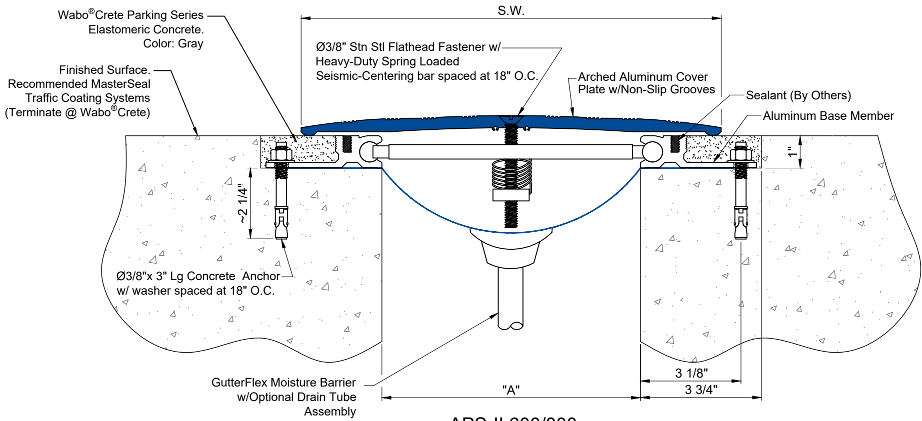
APS-II 600/800 Floor to Floor Condition
