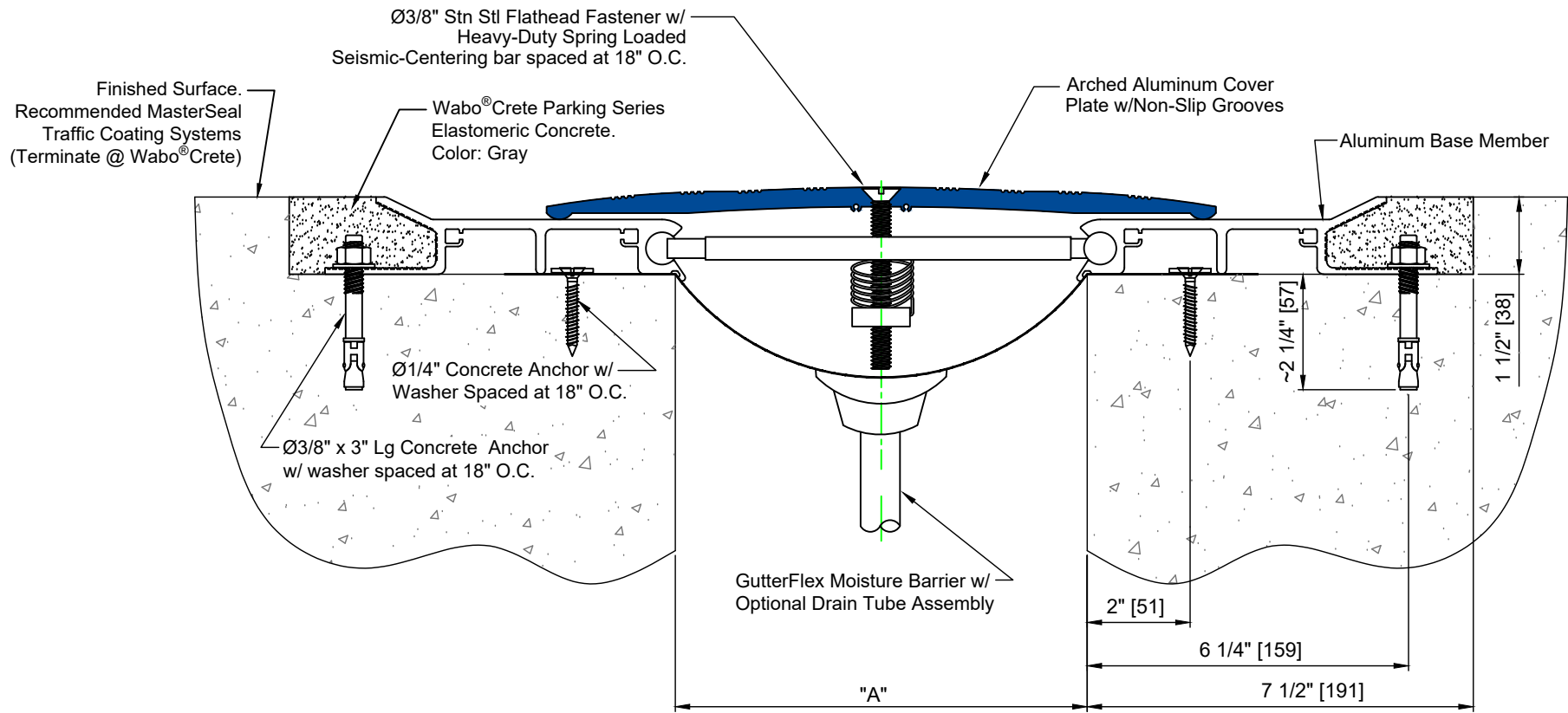
APX-II 600/800 DETAIL FLOOR TO FLOOR CONDITION NOT TO SCALE
