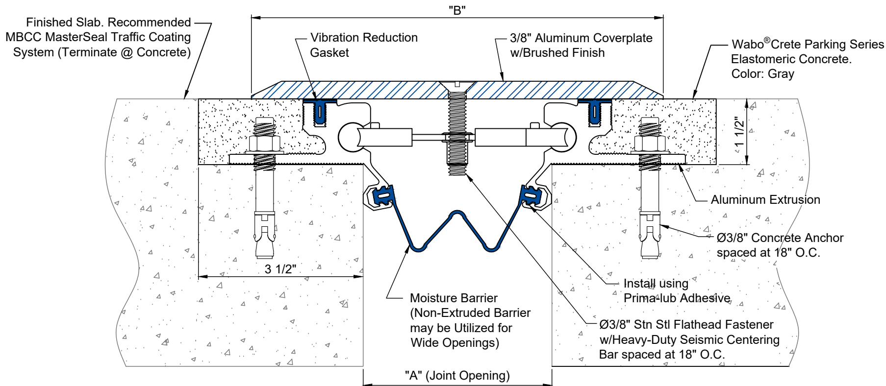
APS-200 THRU APS-1800 DETAIL
